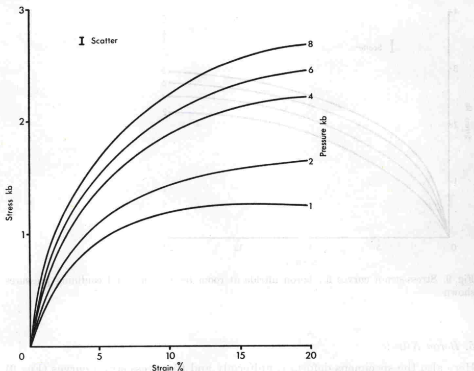
Fig. 10. Stress-strain curves for graphite at room temperature and confining pressures shown
