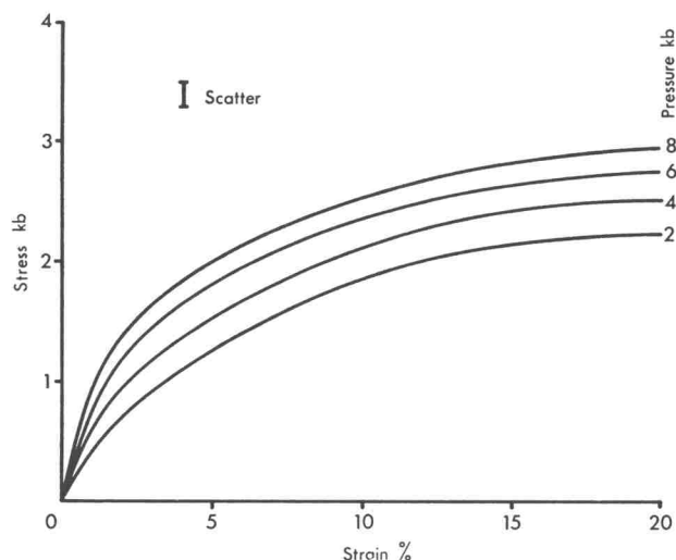
Fig. 9. Stress-strain curves for boron nitride at room temperature and confining pressures shown
